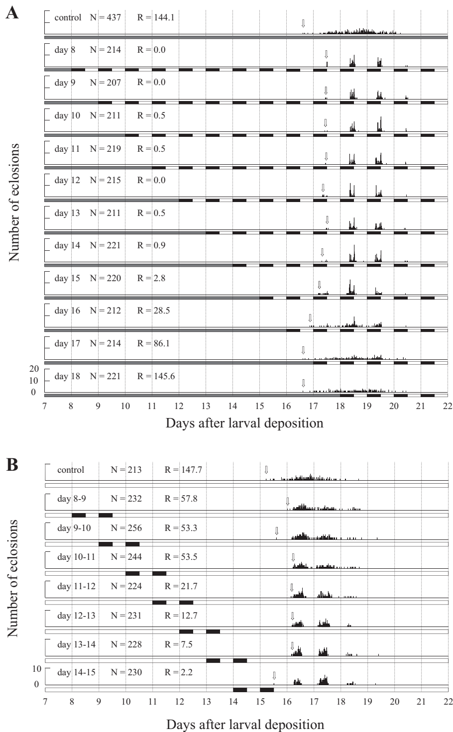
Fig. 2. Effects of temperature cycles on Sarcophaga crassipalpis eclosion rhythms in continuous light. Distributions of adult eclosion are shown at 6 min intervals. (A) Pupae were transferred from a constant temperature of 25°C to temperature cycles at different pupal stages. (B) Pupae under a constant temperature of 28°C were provided with two temperature cycles at different pupal stages. White bar, 28°C; gray bar, 25°C; black bar, 22°C. White arrows indicate start of eclosion.
