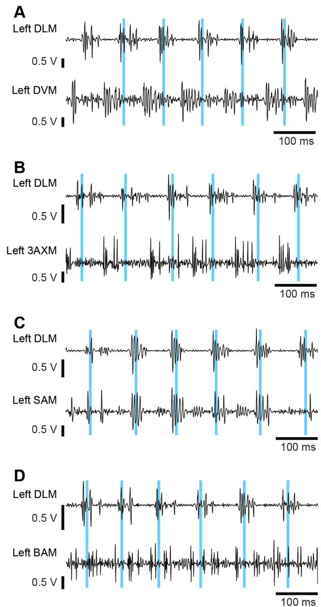
Fig. 5. EMGs of representative flight muscles during a free-flight. (A–D) EMGs of the five muscles were measured sequentially in the same butterfly. The DLM activity is shown as a reference. EMGs of the DVM (A) , 3AXM (B) , SAM (C) , and BAM (D) are shown. Blue vertical bars indicate the wing dorsal stroke reversal timing. The activation phases of these muscles are shown in Fig. 6.
