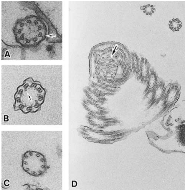
Fig. 6. Transmission electron micrographs of the flagella of spermatozoa from Conger myriaster . (A) Transverse section through the flagellum near to the distal centriole. The two subfibrils were linked to the plasma membrane by radial Y-shape electron-dense bodies (arrow). \times 120,000 . (B) Transverse section through the main flagellum. The inner dynein arms (arrow) are seen. \times 136,000 . (C) Transverse section through the flagellum near the distal tip. \times 136,000 . (D) Cross section of coiled flagella. The flagellum is coiled tightly with about 7–8 strata as counted from the center (arrow) to the periphery. In this case the coil is somewhat bent. \times 55,600 .
