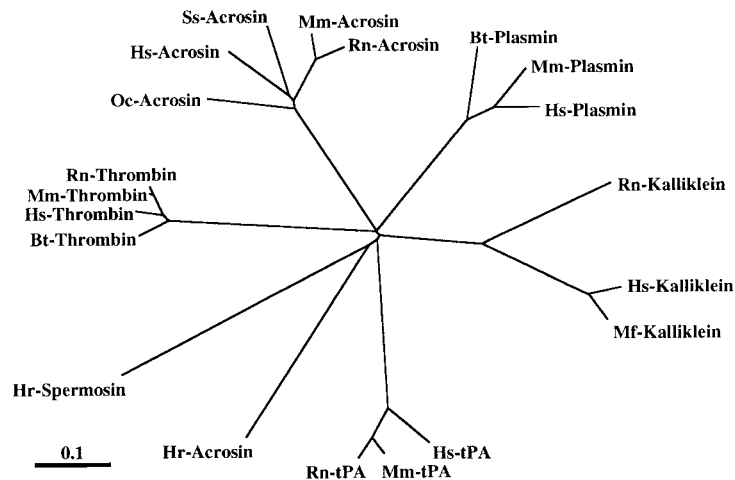
Fig. 5. Dendrogram depicting the relationship between ascidian acrosin, ascidian spermosin and mammalian trypsin family. Clustal W was used to generate alignments of the amino acid sequences of the preproenzyme, which were then displayed with Tree-View. A scale bar indicates the 0.1 amino acid substitutions per residue. The DDBJ/GenBank/EMBL accession numbers of respective proteases are described below. Hr-Acrosin, Halocynthia roretzi (ascidian) acrosin, AB052635; Hr-Spermosin, Halocynthia roretzi (ascidian) spermosin, AB052776; Ss-Acrosin (pig), J04950; Hs-Acrosin (human), Y00970; Mm-Acrosin (mouse), D00754; Oc-Acrosin (rabbit), U05204; Rn-Acrosin (rat), X59254; Hs-Kallikrein (human), M25629; Mf-Kallikrein (monkey), L10039; Rn-Kallikrein (rat), M19648; Bt-Plasmin (bovine), X79402; Hs-Plasmin (human), A22096; Mm-Plasmin (mouse), J04766; Hs-tPA (human), A01465; Mm-tPA (mouse), J03520; Rn-tPA (rat), A19618; Bt-Thrombin (bovine), J100041; Hs-Thrombin (human), J00307; Mm-Thrombin (mouse), M81394; Rn-Thrombin (rat), M81397.
