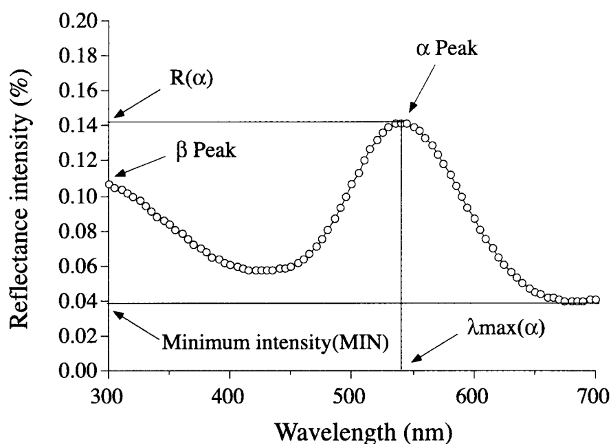
Fig. 2. Representative reflectance spectra of the dorsal surface of two species of dung beetle. Variables extracted from the spectral data (81 points from 300 to 700 nm in 5-nm increments) include \alpha and \beta peak wavelength ( \lambda_{\max}(\alpha) and \lambda_{\max}(\beta) , respectively), reflectance intensity ( R(\alpha) and R(\beta) , respectively), mean intensity, and minimum intensity (MIN).
