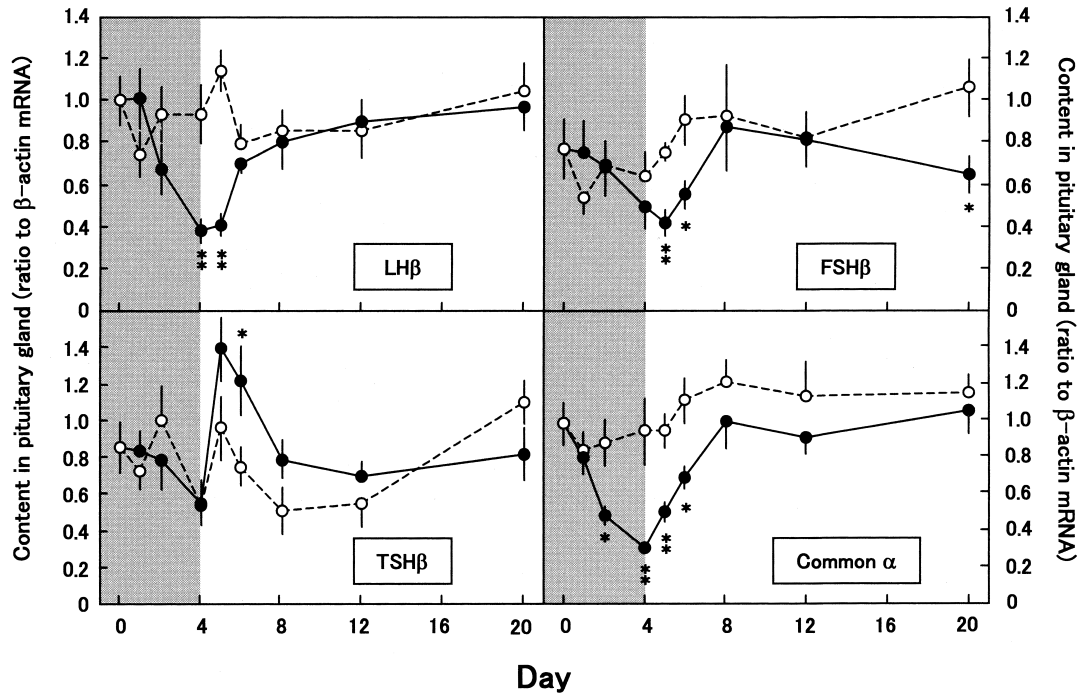
Fig. 3. Changes in pituitary contents of LHβ, FSHβ, TSHβ and common α mRNA in experimental (solid circles with solid line) and control (open circle with broken line) groups. The values are expressed as the ratio to β-actin mRNA content. Circles and bars represent the mean±SEM. Shaded area represents the food deprivation period. Significant differences between the experimental and control groups on the same day are indicated at P<0.05 (*) and P<0.01 (**).
