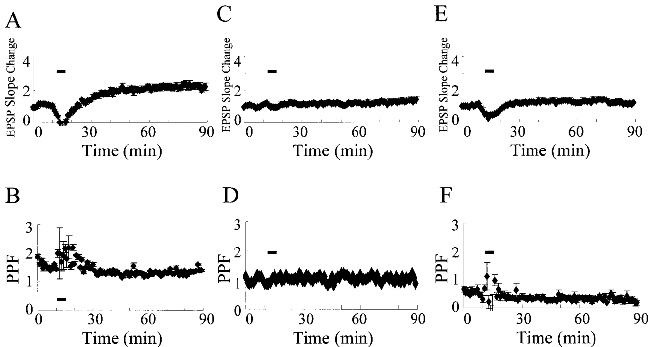
Fig. 2. Ischemia-induced changes of fEPSP slope and PPF ratio. (A and B) Time-dependent changes of fEPSP slope and PPF ratio of the normal condition ( [Ca^{2+}]_o = 2 mM) group, (C and D) time-dependent changes of fEPSP slope and PPF ratio of the higher concentration Ca 2+ ( [Ca^{2+}]_o = 10 mM) applied group, and (E and F) time-dependent changes of fEPSP slope and PPF ratio of the 2 mM 4-aminopyridine (4-AP) added group are shown. Data are expressed as mean±SE. In each case, the control level of fEPSP was normalized to 1. The period of ischemia is expressed as a solid black bar.
