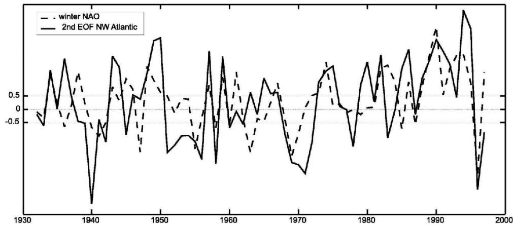
Figure 6. Winter North Atlantic Oscillation (dashed line) coplotted with the second empirical orthogonal function of northwest Atlantic tide-gauge records (solid line).
