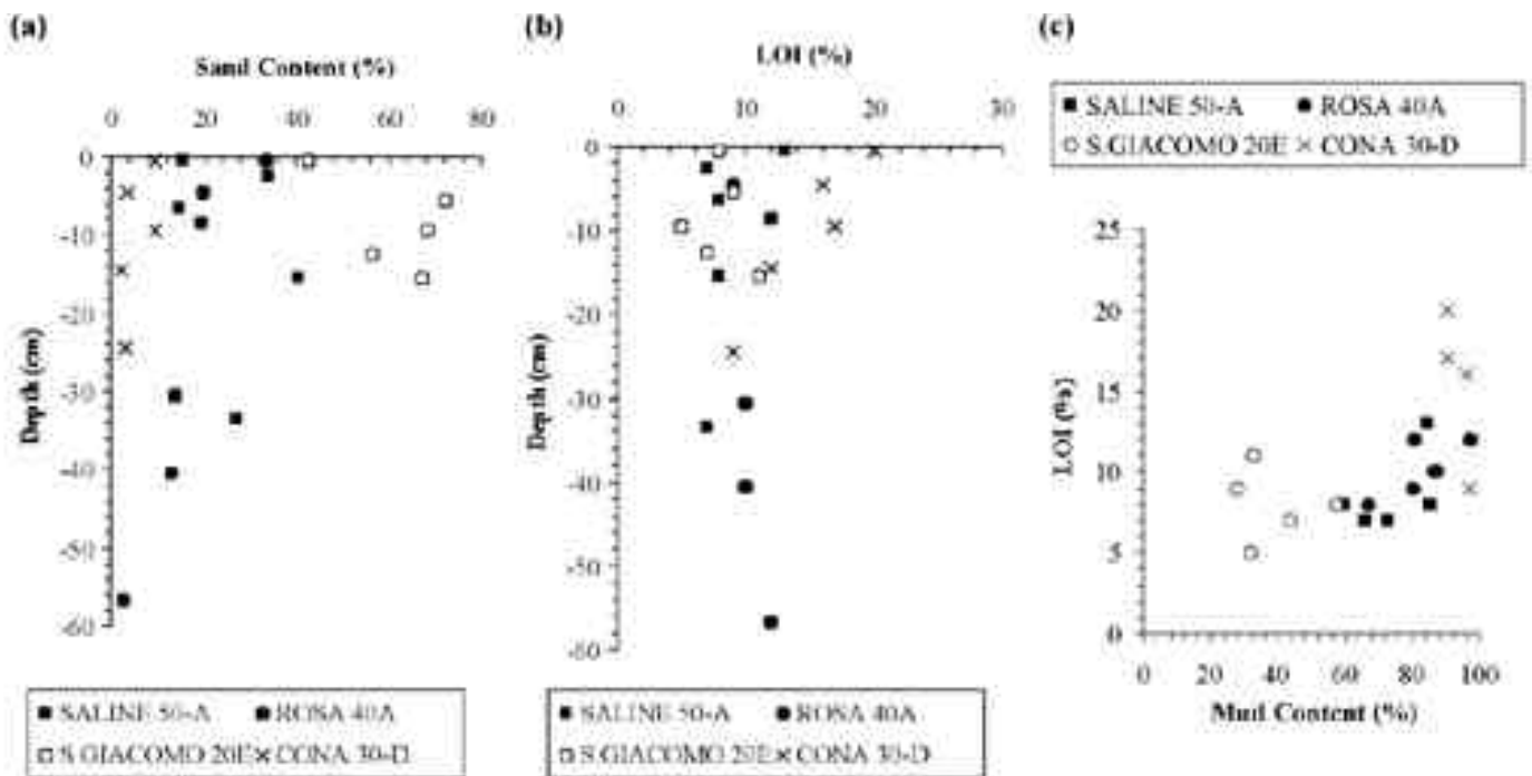
Figure 2. Results of sedimentological analyses: (a) Sand content; (b) Loss On Ignition; (c) Mud content vs LOI.
