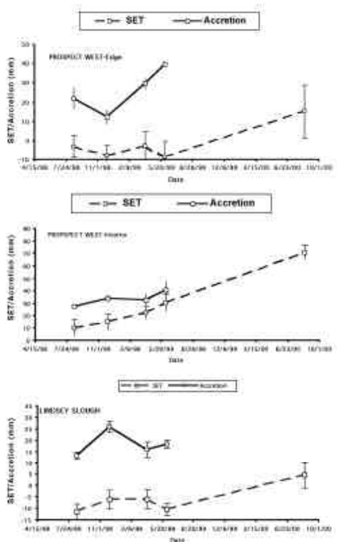
Figure 2. Results of marsh surface accretion and elevation change (SET) measurements at the northern delta study sites (Northern delta sites were not measured in June 1998 because of logistical difficulties).
