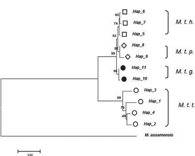
Fig. 2. A phylogenetic tree of mtDNA haplotypes. This figure is a Neighbour Joining tree for 11 haplotypes which were calculated from 44 mitochondrial DNA control region sequences.
