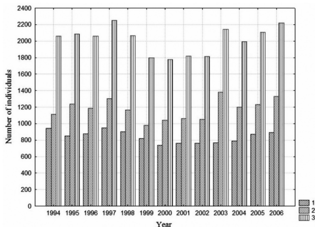
Fig. 1. Main areas of the occurrence of chamois (a) in Bulgaria: Stara Planina Mountain (POP-1), Rhodope Mountains (POP-2), Rila Mountain (POP-3) and Pirin Mountain (POP-4); and absolute numbers (b) of the chamois during the period 1994-2006: (1) – in protected park territories, (2) – partly protected park territories and (3) – all over the territory of Bulgaria.
