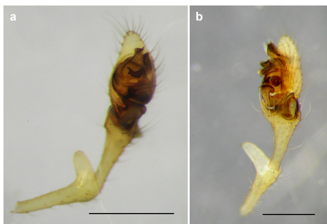
Fig. 5: Male palp of Erigone cristatopalpus from the Ukrainian Carpathians. a. ventral view; b. retrolateral view. Scale bars: 0.5 mm
