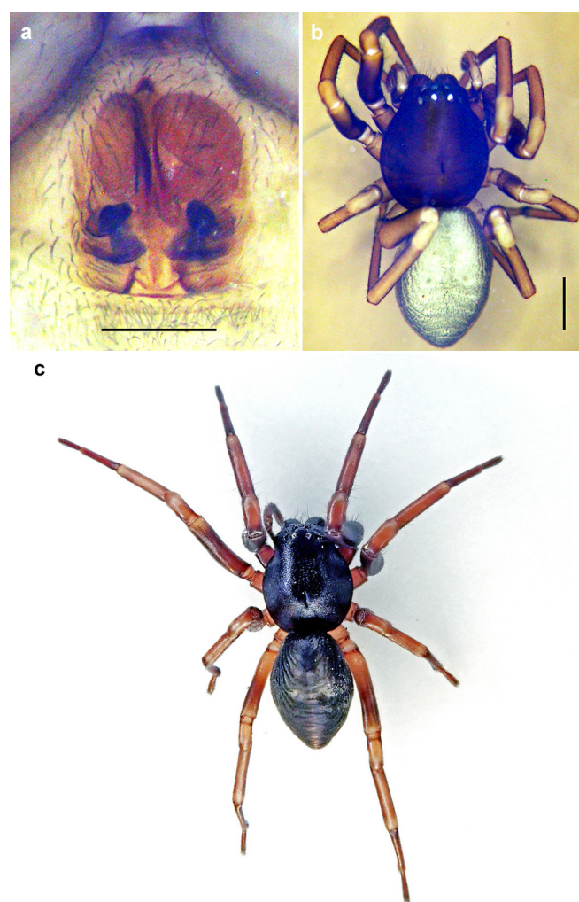
Fig. 6: Females of Cetonana laticeps from the Ukrainian Carpathians (a, b) and Germany (c). a. epigyne; b. general appearance; c. adult specimen ( https://www.inaturalist.org/observations/152067938 ). Scale bars: 0.2 mm (a); 1 mm (b)
