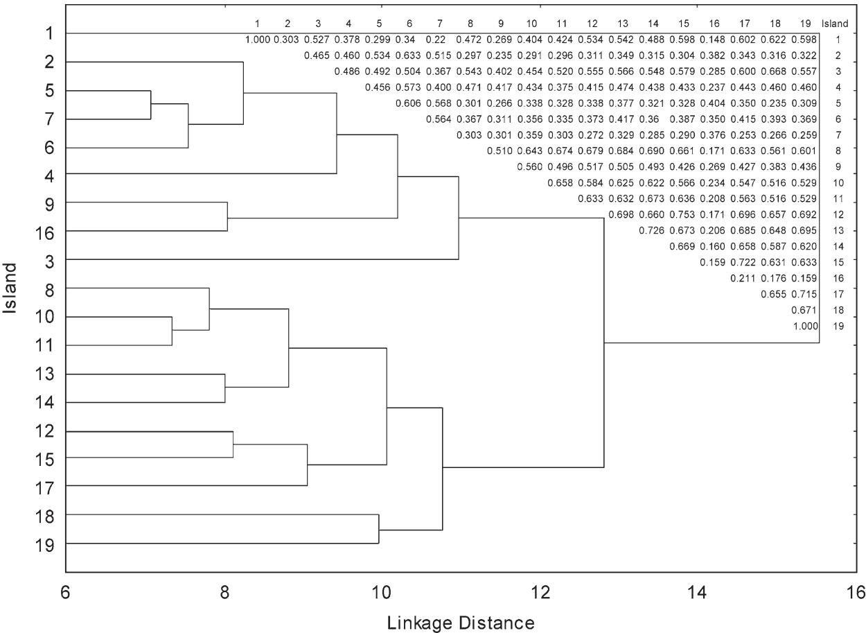
Fig. 2. Hierarchical cluster analysis showing floristic relations between the Echinades islets (linkage method: complete linkage. Euclidean distances). The table on the upper right side of the dendrogram presents floristic cross-correlations (beta-diversity) between the studied islets by means of the Sørensen similarity coefficient. – Abbreviations are as in Table 1.
