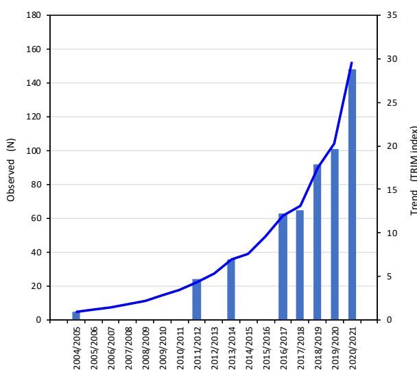
Fig. 2. Variation of wintering Rhinolophus ferrumequinum bats in the period 2004/2005 - 2020/2021.
