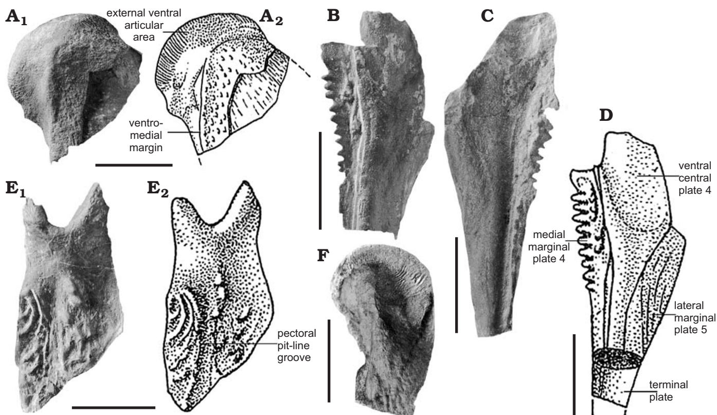
Fig. 7. Dermal plates of antiarch placoderm Asterolepis sp. 1, from Hingeon (Namur Province), Upper Givetian, Devonian. A. IRSNB P.1460, CV1, external view; photograph ( A 1 ), explanatory drawing ( A 2 ). B. IRSNB 1462a, distal part of the pectoral fin, external view. C. IRSNB 1462b, distal part of the pectoral fin, external view, counterpart of IRSNB 1462a. D. Drawing based on IRSNB 1462a and b, distal part of the pectoral fin, external view. E. IRSNB P.1463, MM1, external view; photograph ( E 1 ), explanatory drawing ( E 2 ). F. IRSNB P.1461a, CV1, internal view. Drawings from Gross 1965. Scale bars 10 mm.
