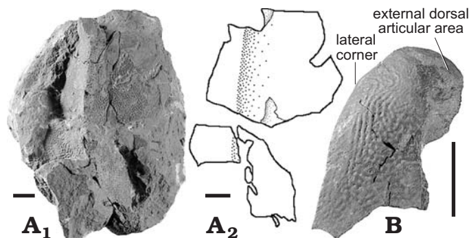
Fig. 8. Dermal plates of antiarch placoderm Asterolepis sp. 2., from Mazy (Namur Province), Givetian, Devonian. A. IRSNB P.9260, unassigned plate, external view; photograph ( A 1 ), explanatory drawing ( A 2 ). B. IRSNB P.9259, CD1, external view. Scale bars 10 mm.
