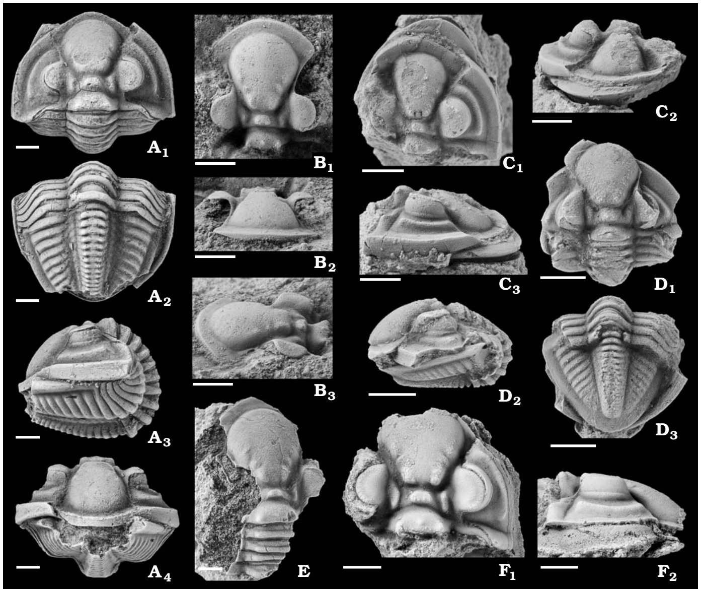
Fig. 4. Ditomopygine trilobite Simulopaladin tridentifer sp. nov. from Kungurian–Roadian (Permian) of Wadi Khawr al Jaramah, Oman. A. Holotype, enrolled complete specimen, NHMUKPI It 29096; cephalon in dorsal view ( A_1 ); pygidium and half thorax in dorsal ( A_2 ), lateral ( A_3 ), and anterior ( A_4 ) views. B. NHMUKPI It 29097; cranidium in dorsal ( B_1 ), anterior ( B_2 ), and lateral ( B_3 ) views. C. NHMUKPI It 29100; incomplete cephalon in dorsal ( C_1 ), anterior ( C_2 ), and lateral ( C_3 ) views. D. Enrolled specimen, NHMUKPI It 29101; cephalon in dorsal ( D_1 ) and lateral ( D_2 ) views; pygidium and half thorax in dorsal view ( D_3 ). E. NHMUKPI It 29099; cranidium and 4 thoracic segments in dorsal view. F. NHMUKPI It 29095; cephalon with cuticle showing occipital tubercles in dorsal ( F_1 ) and lateral ( F_2 ) views. Scale bars 2.5 mm.
