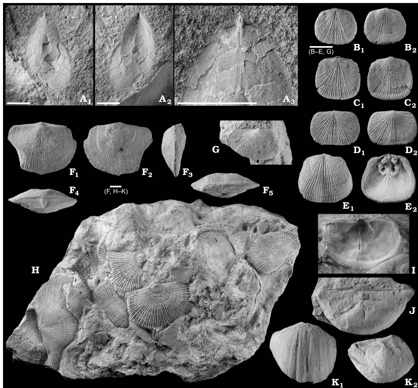
Fig. 2. Middle to Latest Famennian brachiopods from Kowala. A. Barroisella sp. The bivalved specimen ZPAL Bp 57/70a showing strongly exfoliated ventral valve (ventral internal mould) and interior of dorsal valve (lower right) (A 1 ) and its counterpart ZPAL Bp 57/70b (A 2 ); enlargement of the posterior region of the ventral valve showing pseudointerarea and elongated median muscle scar (A 3 ). B–E. Aulacella interlineata (Sowerby, 1840). B–D. Three shells ZPAL Bp 57/4a, 4b, and 86, respectively, in dorsal (B 1 , C 1 , D 1 ) and ventral (B 2 , C 2 , D 2 ) views showing variability in the shell outline. E. Dorsal valve ZPAL Bp 57/5 exterior (E 1 ) and interior (E 2 ). F, H, I. Schellwienella pauli (Gallwitz, 1932). F. Slightly destroyed shell ZPAL Bp 57/20 in dorsal (F 1 ), ventral (F 2 ), lateral (F 3 ), posterior (F 4 ), and anterior (F 5 ) views. H. Limestone block ZPAL Bp 57/103 with accumulation of shells of S. pauli . I. Interior of ventral valve ZPAL Bp 57/100. G. Productida indet., mould ZPAL Bp 57/7 of exfoliated dorsal valve. J. Productida indet. Posterior view of mostly decorticated and slightly crushed dorsal valve ZPAL Bp 57/8. K. Mesoplica sp. Ventral valve ZPAL Bp 57/1 in ventral (K 1 ) and posterior (K 2 ) views. Scale bars 5 mm.
