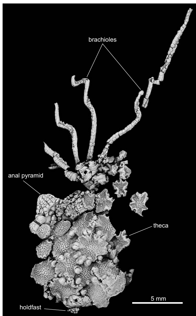
Fig. 1. Holotype (MGM2005K) of gogiid echinoderm Alaniscystis andalusiae Ubaghs and Vizcaïno, 1991 from the lower Cambrian of the Ossa Morena zone (South Spain). Photograph of latex cast whitened with \text{NH}_4\text{Cl} .
