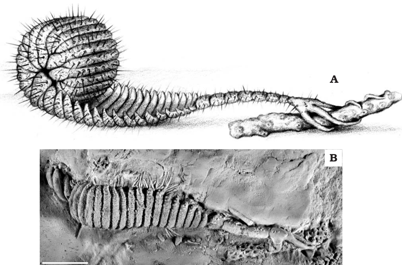
Fig. 7. Ammonocrinus leunissenii sp. nov. A. Reconstruction of a “encased runner-type” of A. leunissenii sp. nov. attached to a tabulate coral (model); the spined specimen dwelled enrolled on the muddy seafloor. B. The original (GIK-2102) from the Eifel (locality 6, Appendix 1), Germany, Lower Givetian (Middle Devonian); showing slightly compressed proximal mesistele. A not to scale, B scale bar 10 mm.
