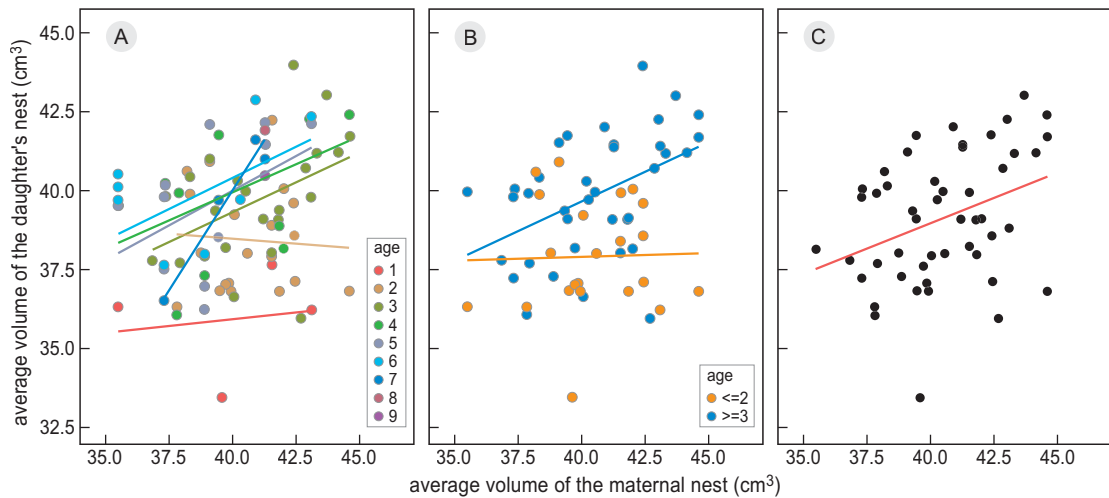
Figure 3. The relationship between average egg volume of the maternal nest and average egg volume of the daughter's nest, with average egg volume of the daughters (A) given at each age for every daughter, (B) averaged into two different age categories for every daughter, and (C) averaged for each daughter across her attempts at all ages. Heritability is estimated from relationship (C): Y = 26.07 + 0.32 \times X , R^2 = 0.11 , n = 49 .
