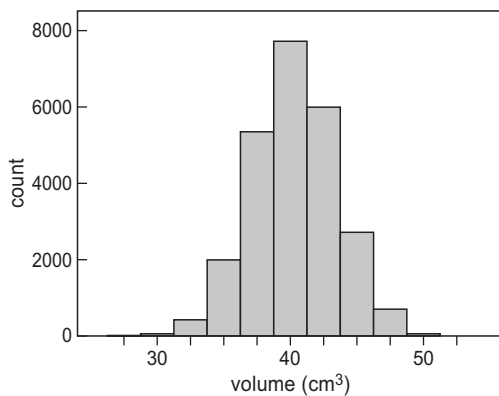
Figure 1. Frequency distribution of 25,148 egg sizes measured in southwest Friesland between 2004–2018. Three eggs with a volume larger than 55 cm 3 (55.04 cm 3 , 55.11 cm 3 and 62.68 cm 3 , respectively), are omitted from this figure for graphical purposes.
