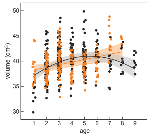
Figure 2. The relationship between egg volume and age for Godwits in southwest Friesland. This graph shows the raw data used in the analysis with body condition included (Model 3, orange dots) and without body condition included (Model 3B, orange + black dots combined). It also shows the modelled estimates and standard errors from Model 3 (orange line, linear relationship) and Model 3B (black line, quadratic relationship).
