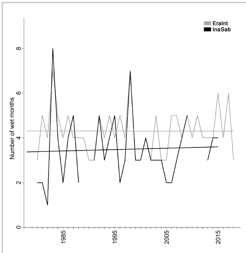
FIGURE S1 Annual duration of the rainy season (Data source: INAMHI, EraInterim)
